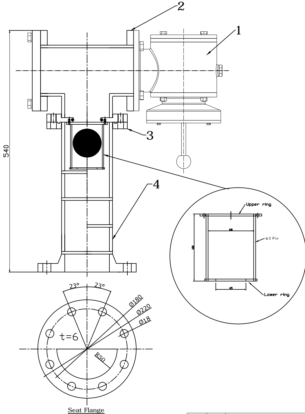
Seat Flange
